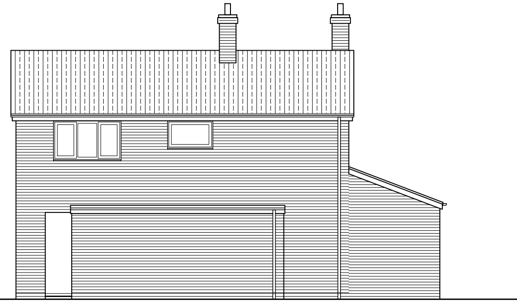
SIDE ELEVATION 1:100
