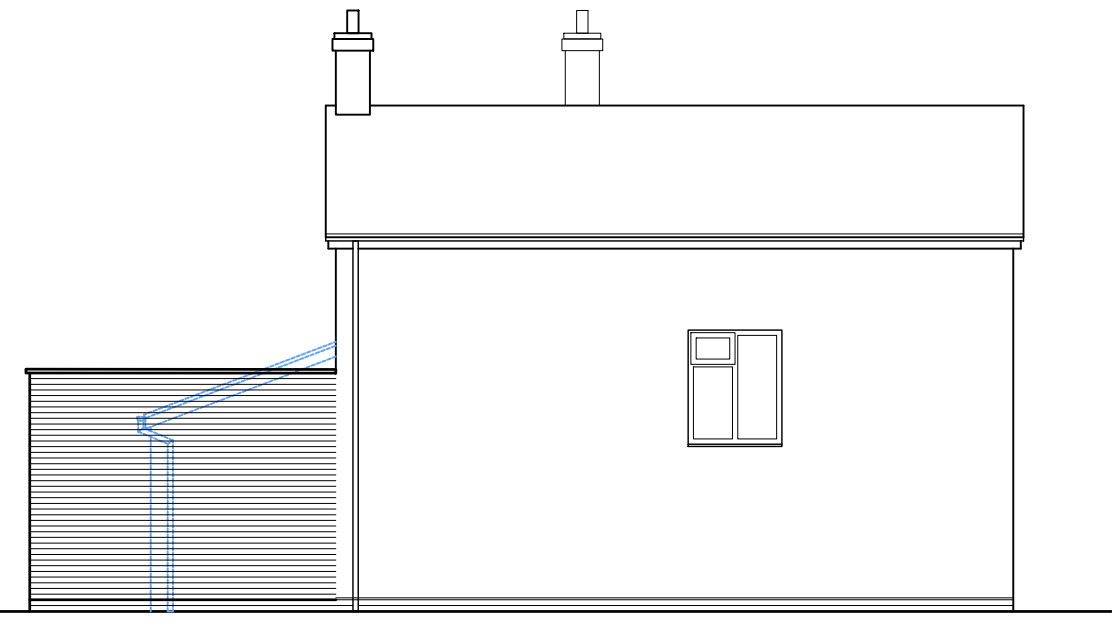
SIDE ELEVATION 1:100
