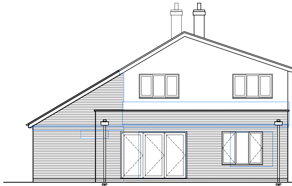
REAR ELEVATION 1:100
