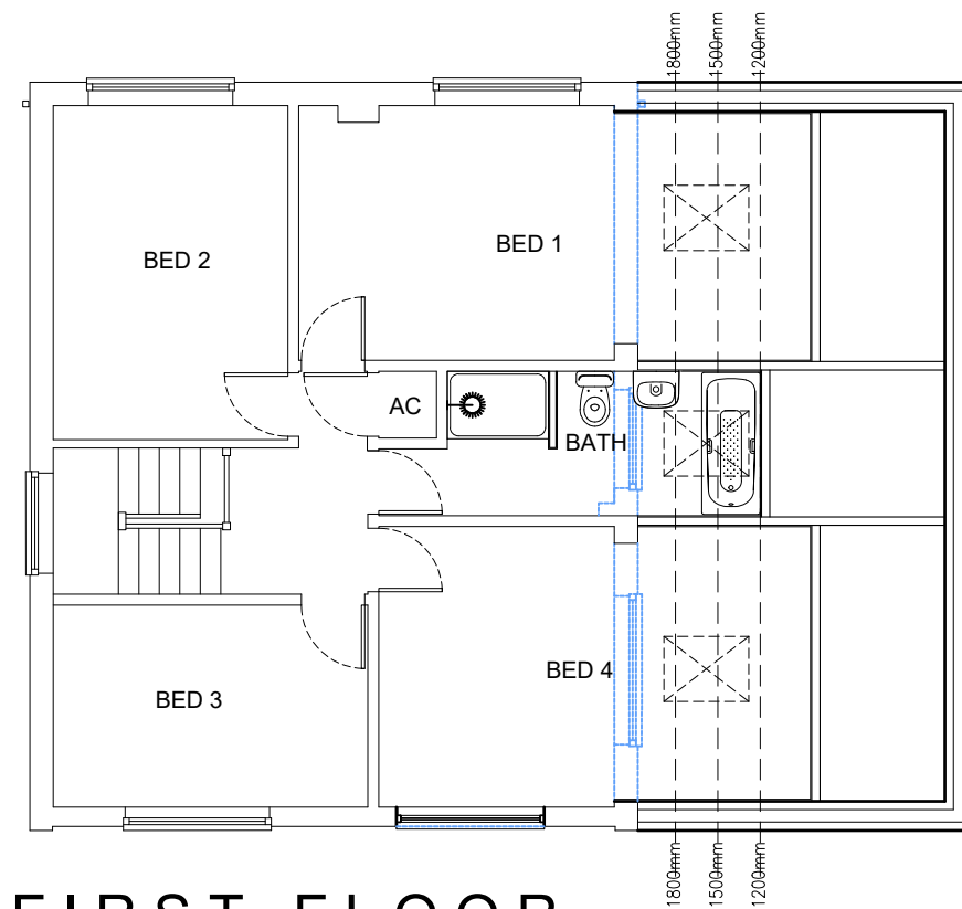
FIRST FLOOR 1:100
