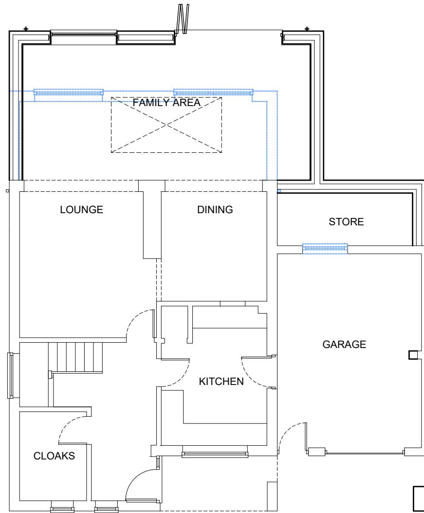
GROUND FLOOR 1:100
