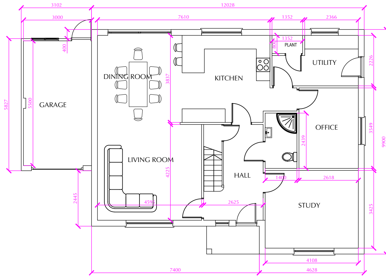
GROUND FLOOR PLAN PLOT 1
