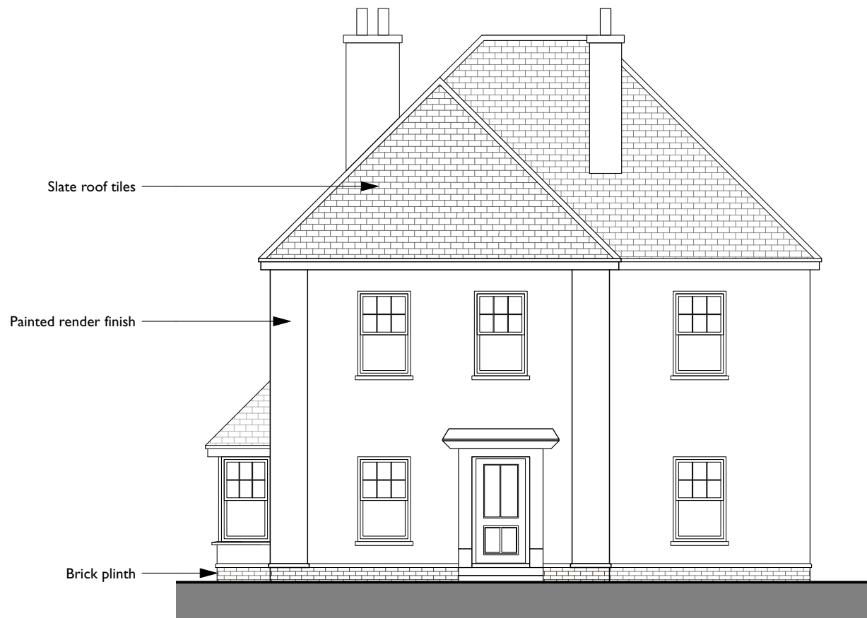
00 - Proposed front elevation 1:100@A3
