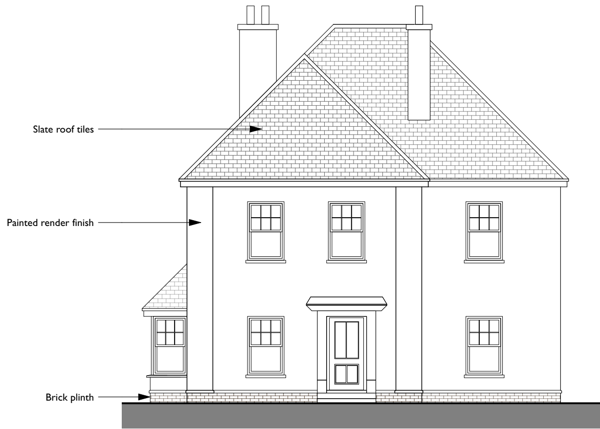
00 - Existing front elevation 1:100@A3
