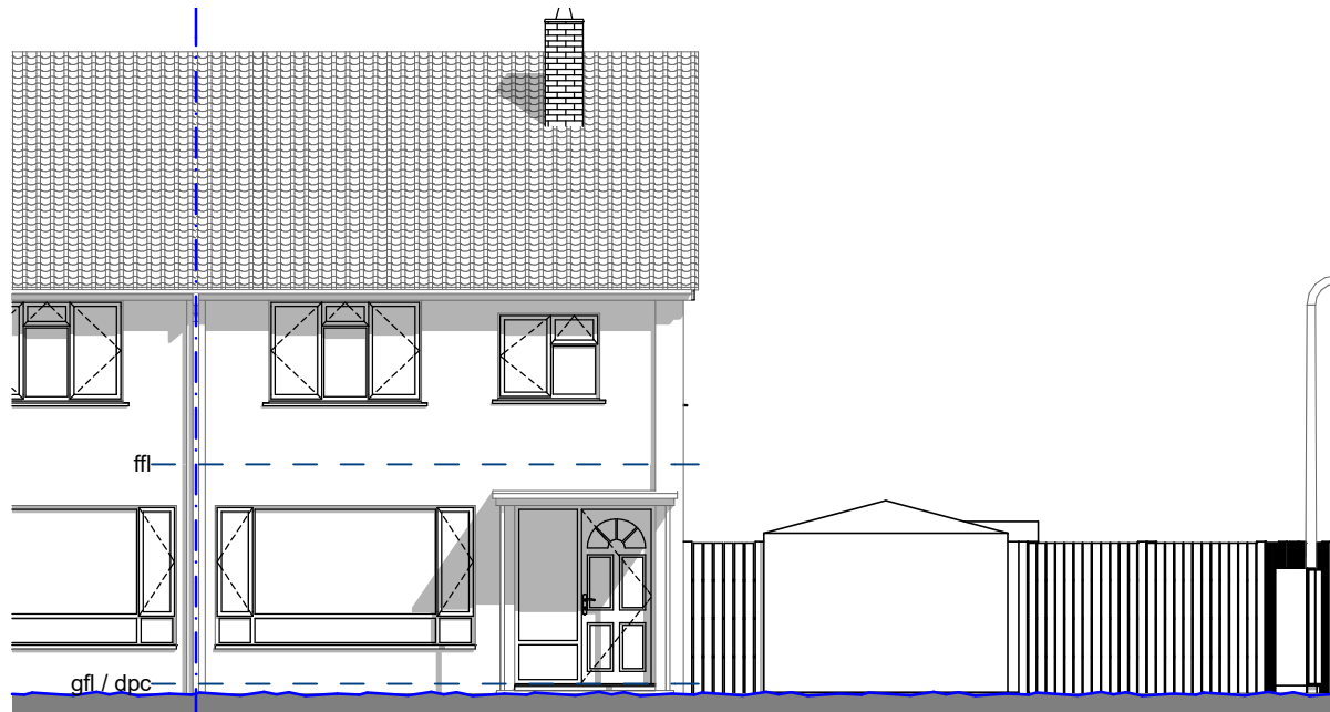
E-01 Front (North) Elevation 1:100
