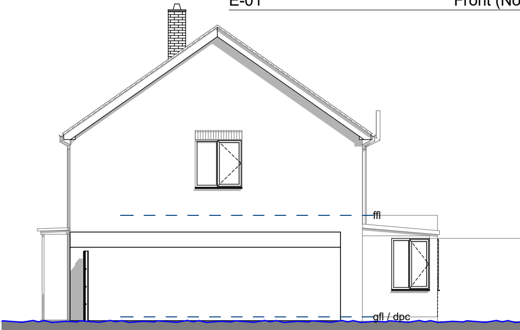
E-02 Side (West) Elevation 1:100
