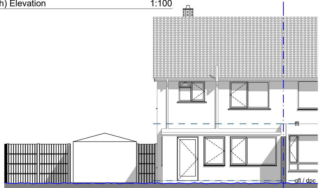
E-03 Rear (South) Elevation 1:100
