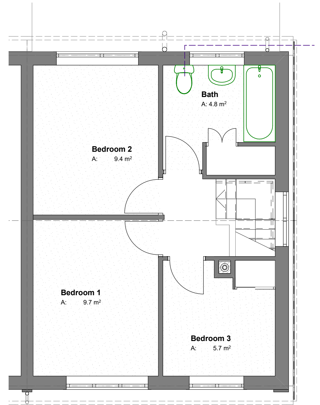
1. First Floor - Existing 1:50
