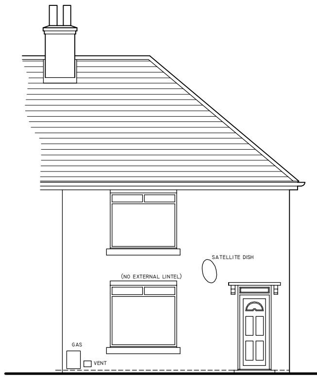
SOUTH WEST ELEVATION Scale 1:100 @ A3
