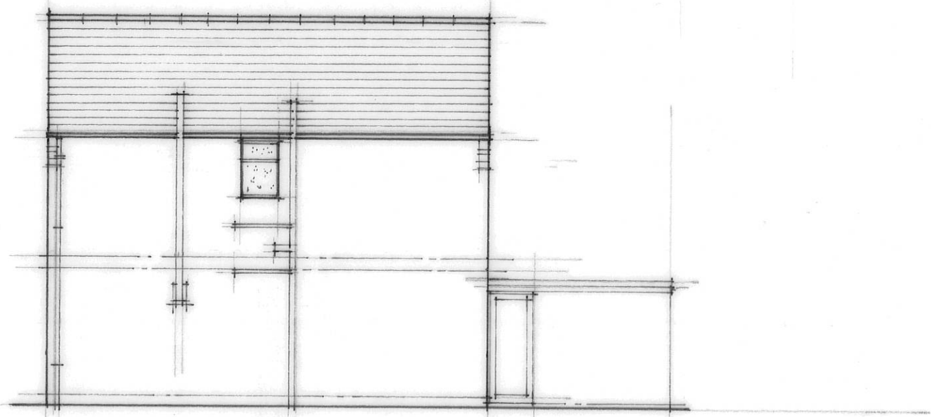
SIDE ELEVATION
