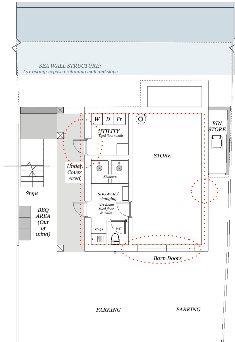
PROPOSED LOWER GROUND FLOOR PLAN
