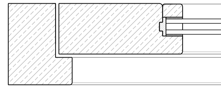
Higher Horizontal Door Section - Scale: 1:2
