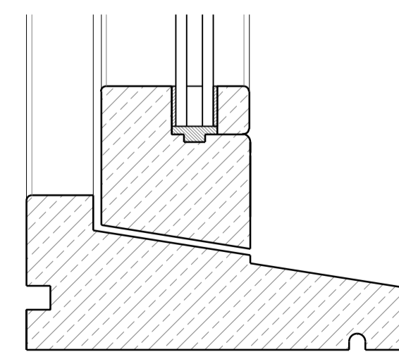
Vertical Window Section Scale: 1:2
