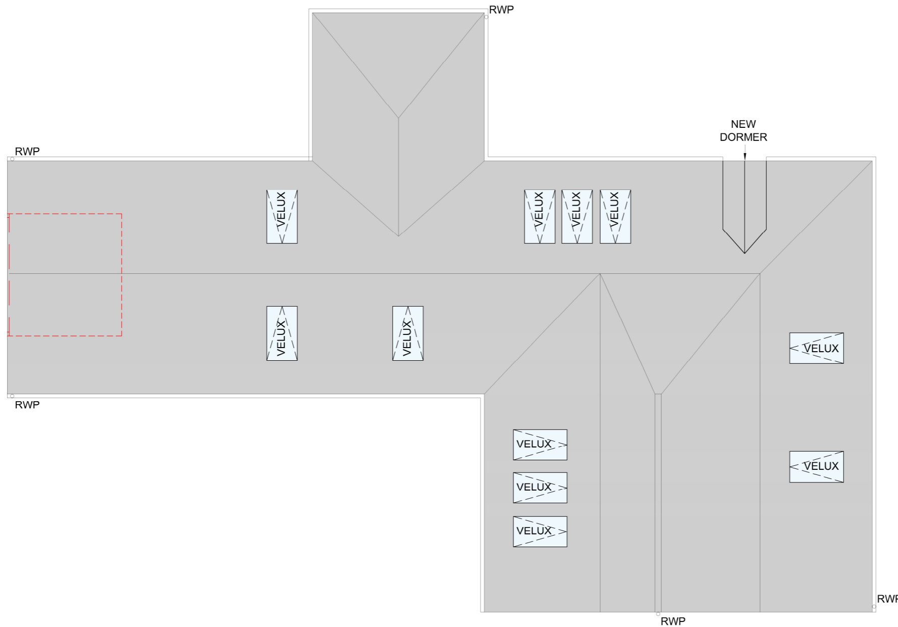
Proposed Roof Plan Scale 1:100 @ A3
