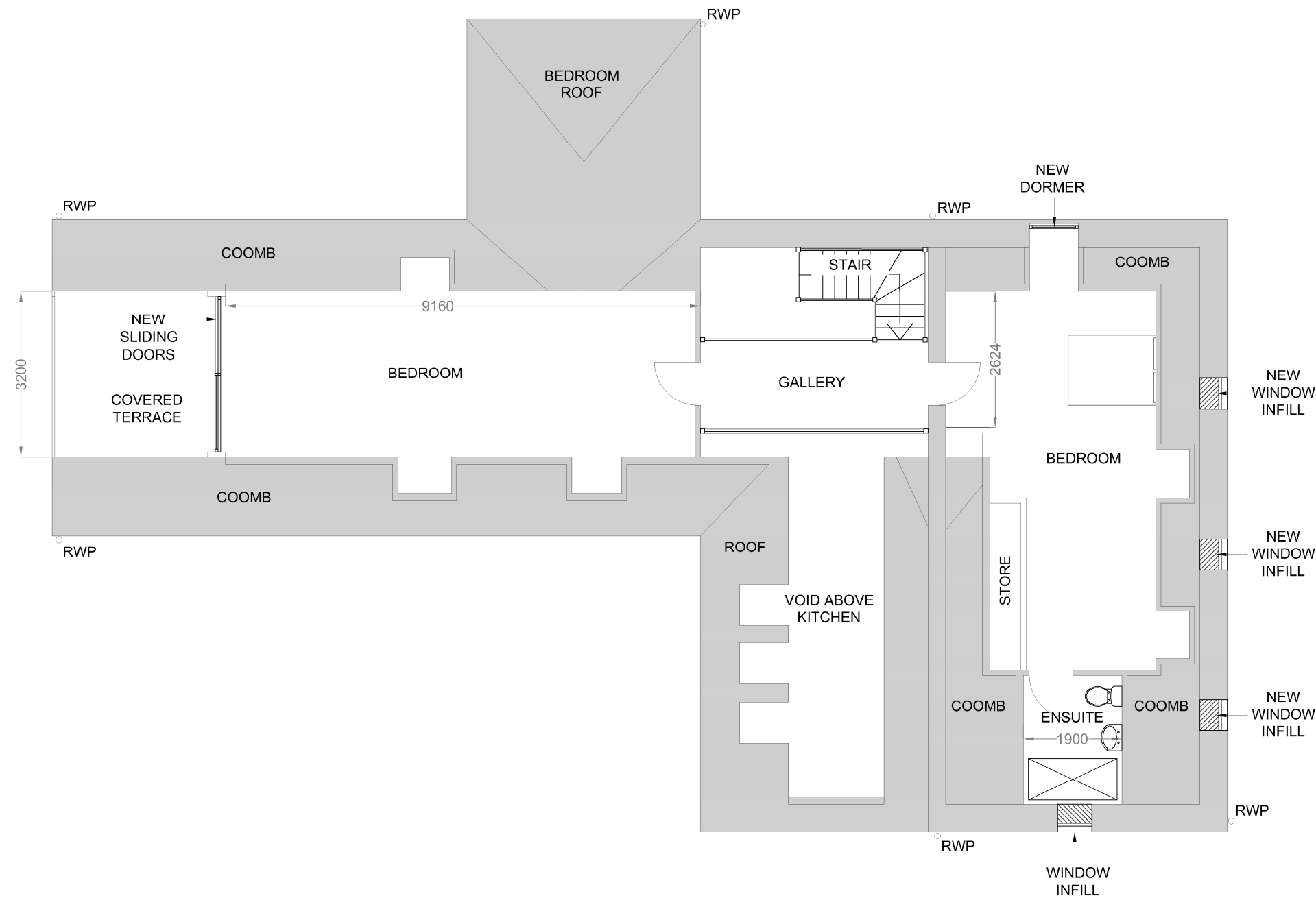
Proposed First Floor Plan Scale 1:100 @ A3
