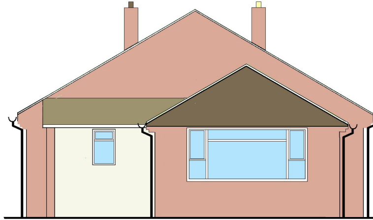
EXISTING ELEVATION - WEST
