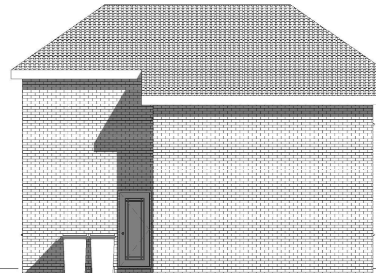
4 South East 1:100
