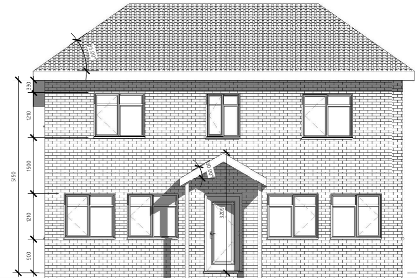
2 North West 1:100
