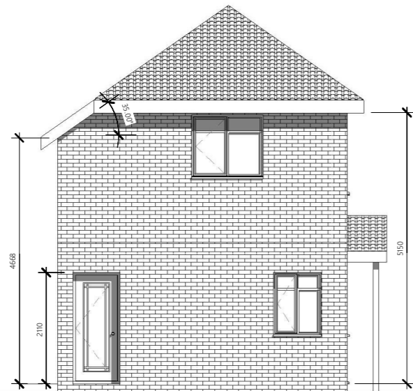
1 North East 1:100
