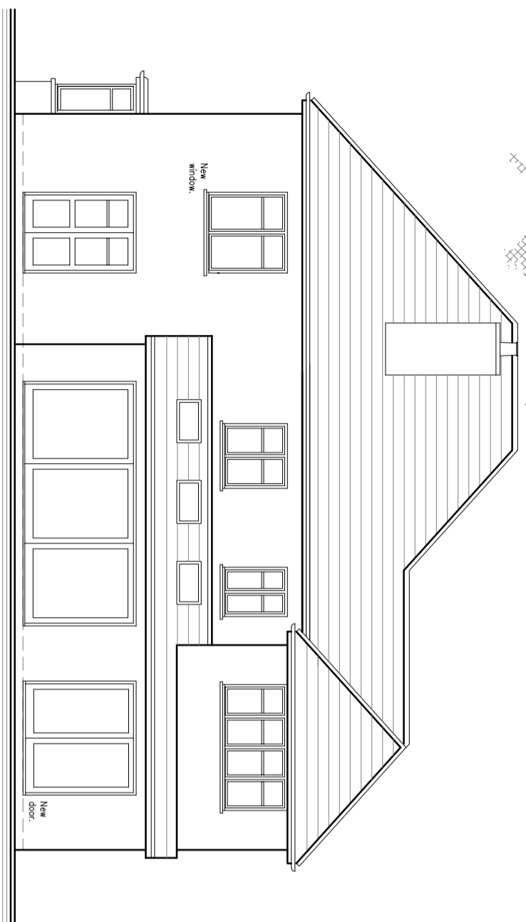
Proposed East Facing Elevation (Rear)
