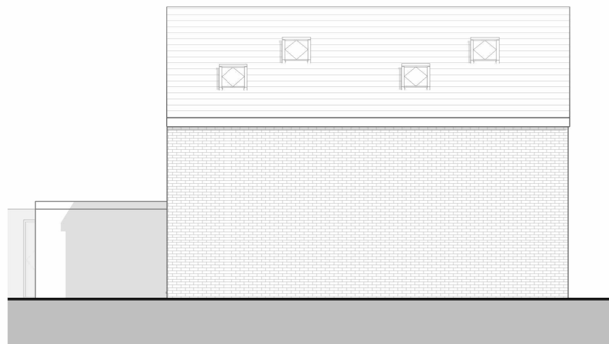
West Elevation
