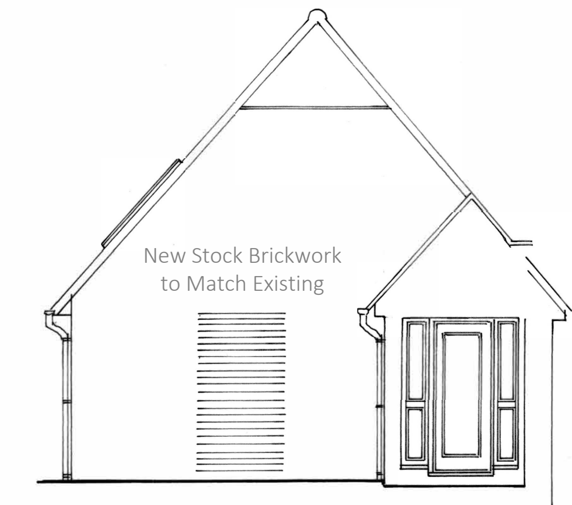
SOUTHELEVATION 1:50
