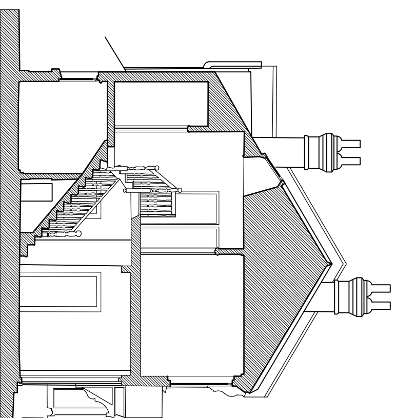
SECTION
