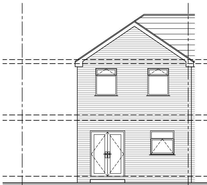
FRONT ELEVATION 1:100
