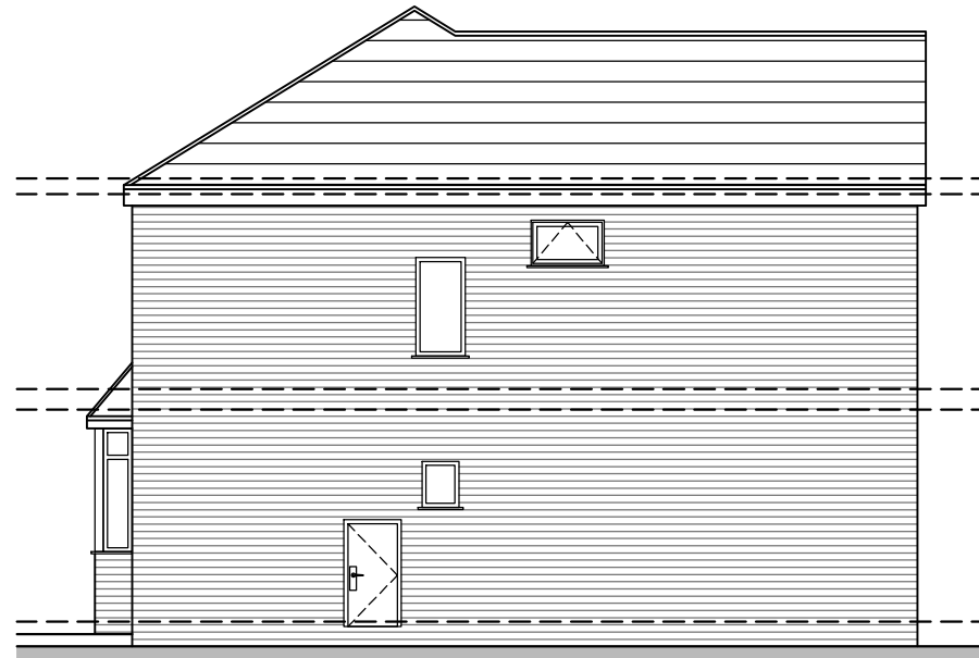
FRONT ELEVATION 1:100
