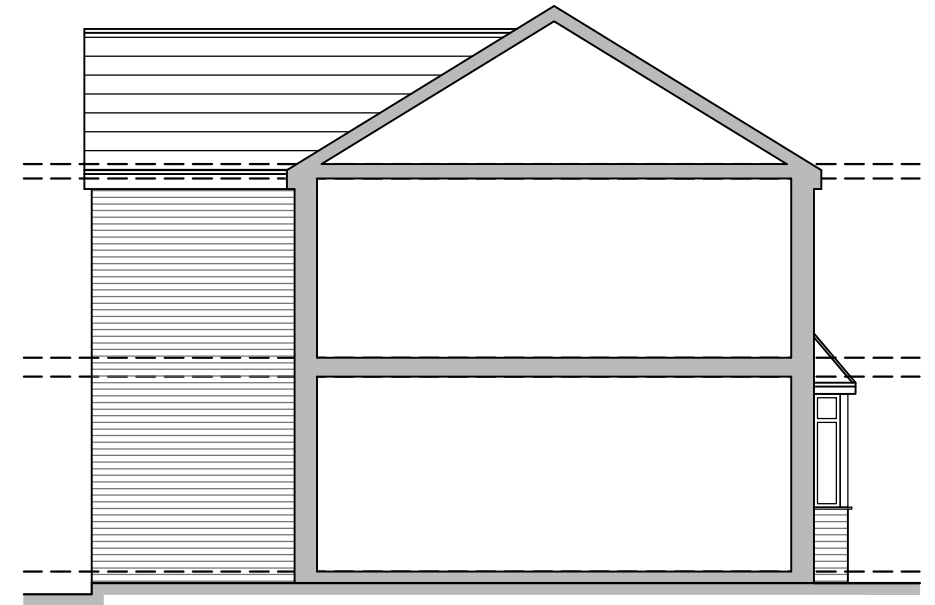
FRONT ELEVATION 1:100
