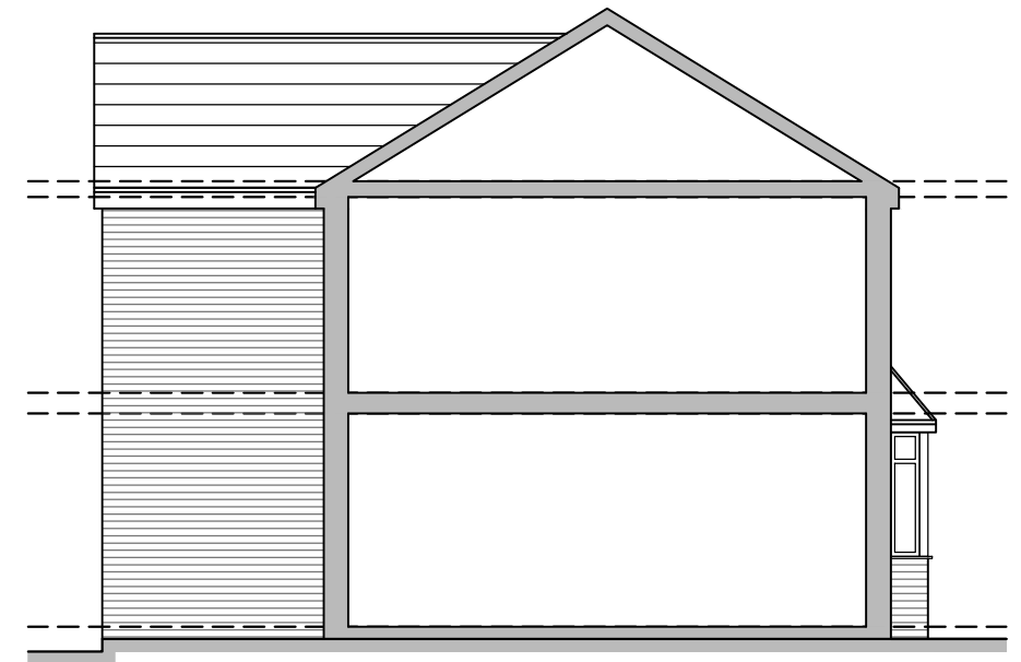
FRONT ELEVATION 1:100
