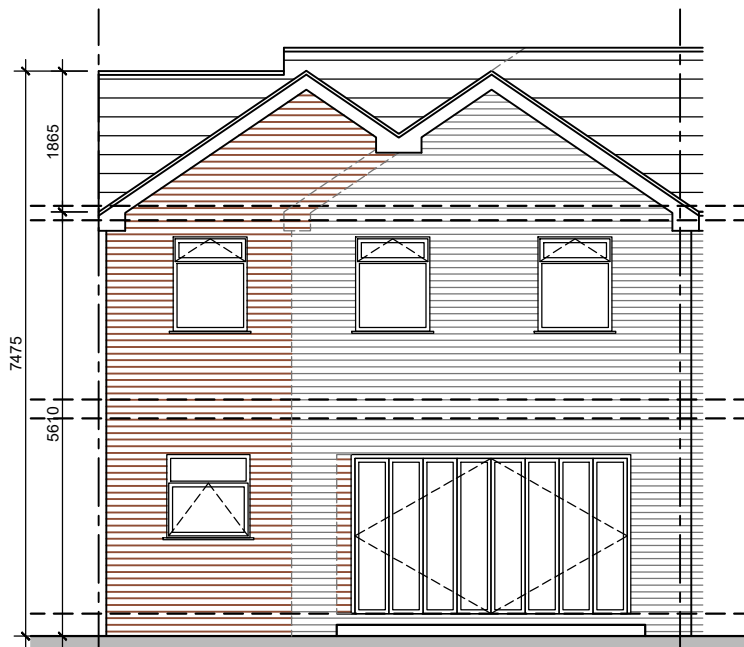
FRONT ELEVATION 1:100
