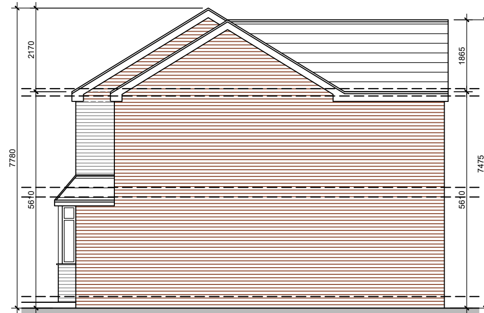
FRONT ELEVATION 1:100
