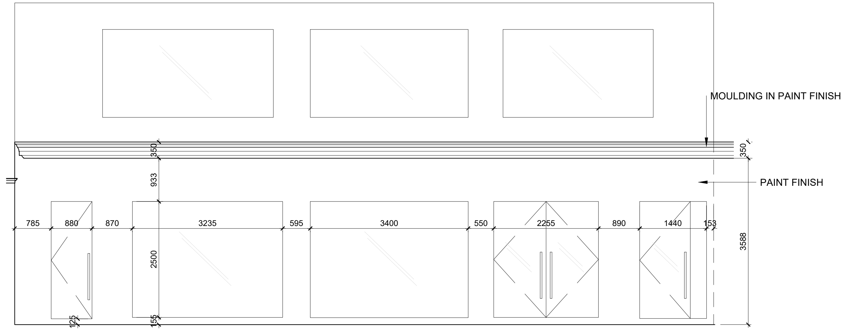
1 EXISTING FACADE 1:50@A3
