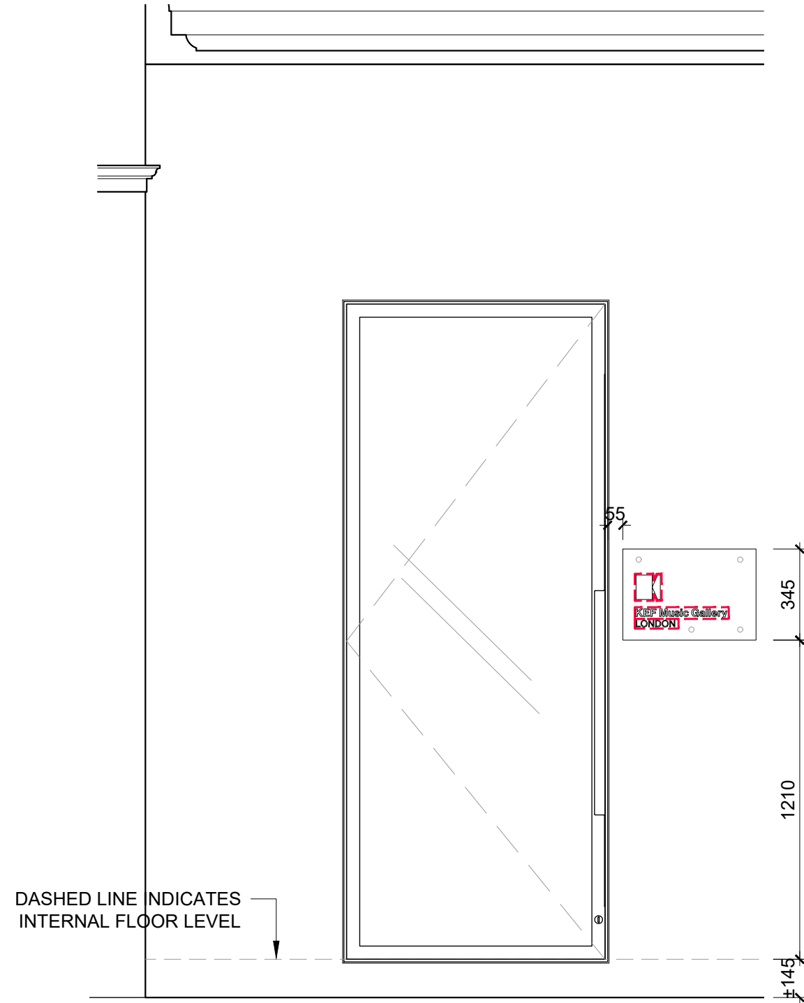
1 FRONT ELEVATION 1:20
