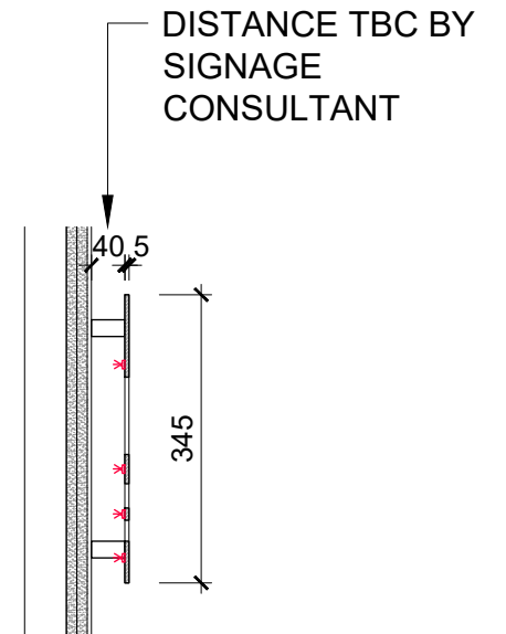
3 SECTION Signage Detail 1:5@A1
