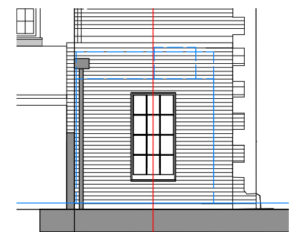
ELEVATION 2 SUMMER ROOM 1:100 ALSO REFER OVERALL ELEVATION
