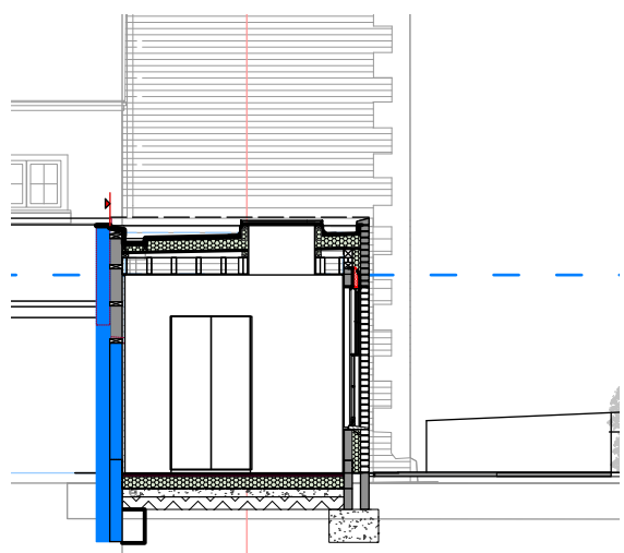
CROSS SECTION SUMMER ROOM 1:100
