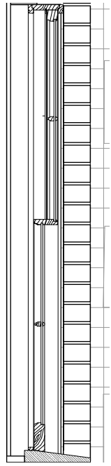
SECTION DETAIL SASH 1:20
