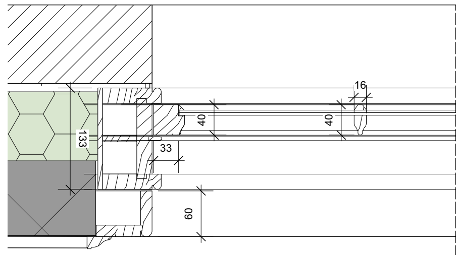
PLAN DETAIL - SASH TYPICAL SASH WINDOW 1:5
