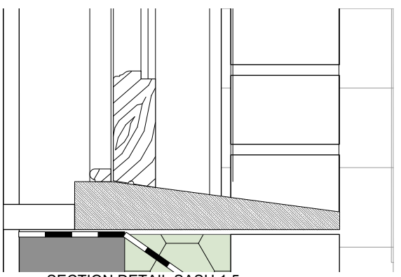
SECTION DETAIL SASH 1:5
