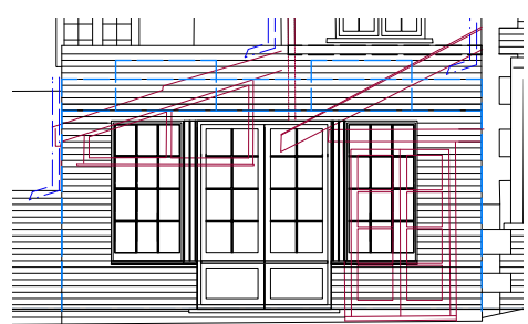
ELEVATION 1 SUMMER ROOM 1:100 ALSO REFER OVERALL ELEVATION
