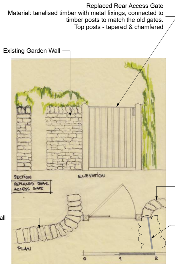
3 Plan & Elevation Replaced Rear Gate 1:50
