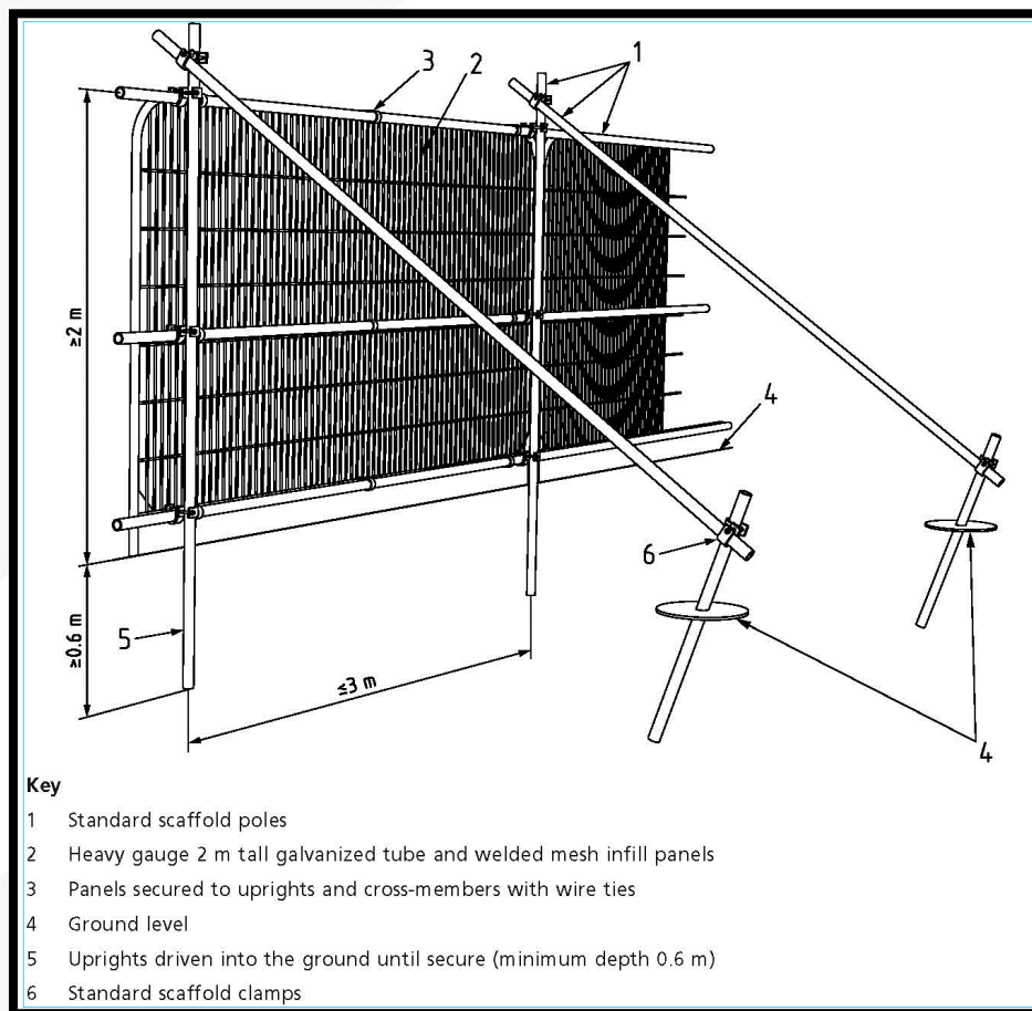
Figure 3: Default specification for protective barrier fencing (BS5837).
