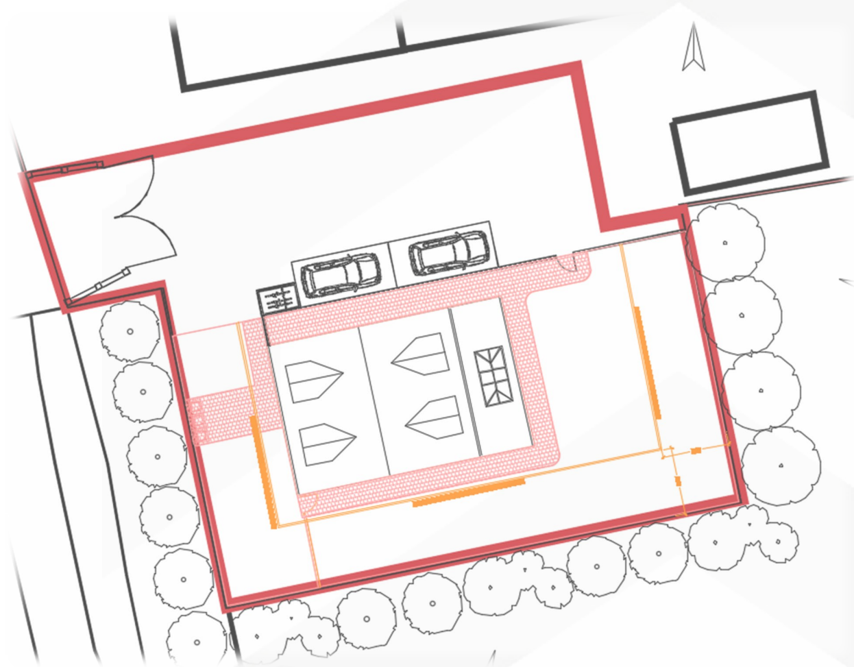
Figure 3: Proposed scheme. Drawing number Y1481/2023/04 (Lyondale Planning & Design).
