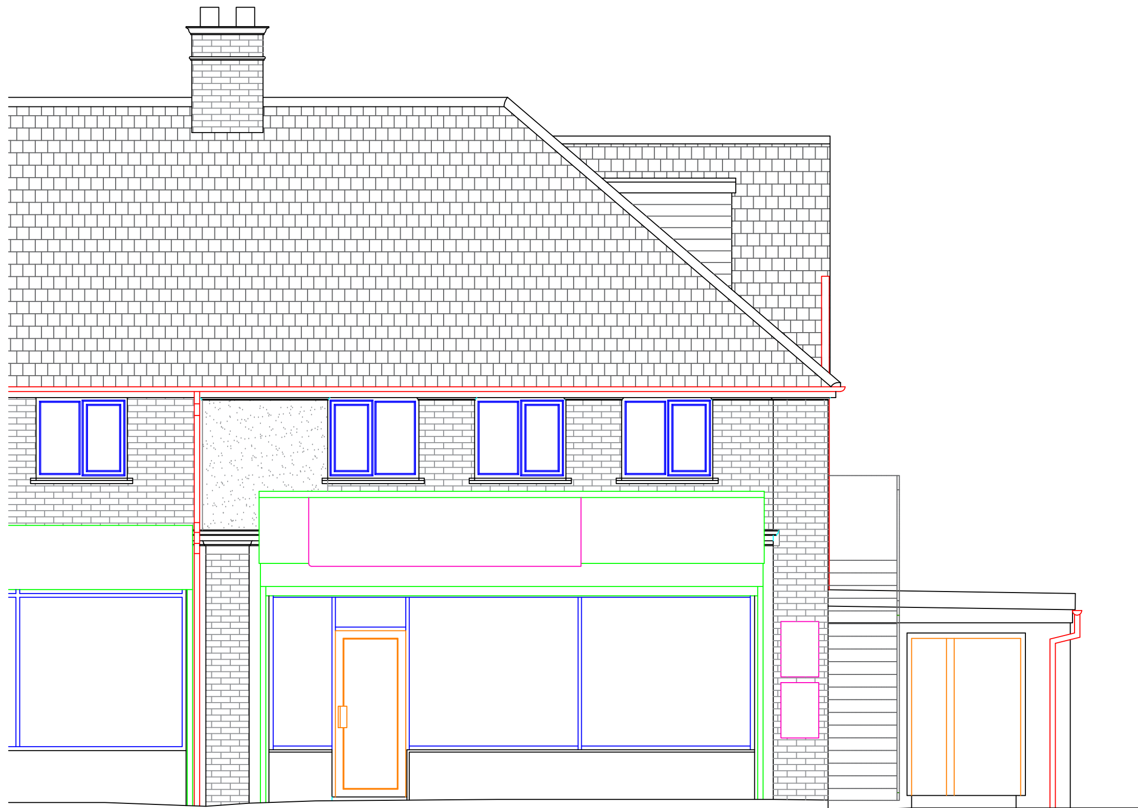
Elevation 1 (viewed from Occupation Road)
