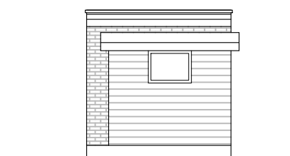
EXISTING FRONT (EAST) ELEVATION
