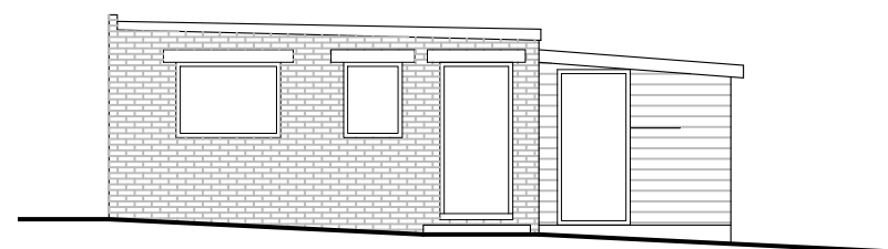
EXISTING SIDE (NORTH) ELEVATION
