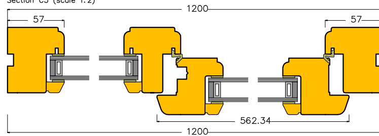
Section C3 (scale 1:2)
