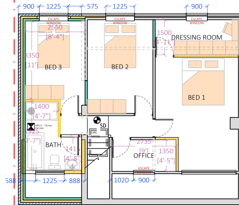
PROPOSED FF PLAN 1:100
