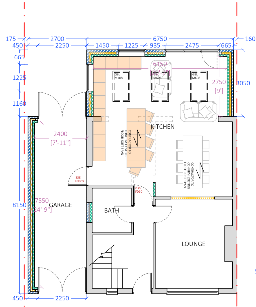
PROPOSED GF PLAN 1:100
