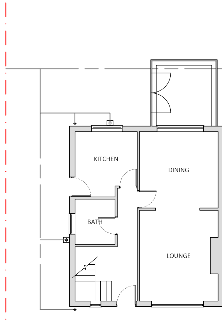
EXISTING GF PLAN 1:100
