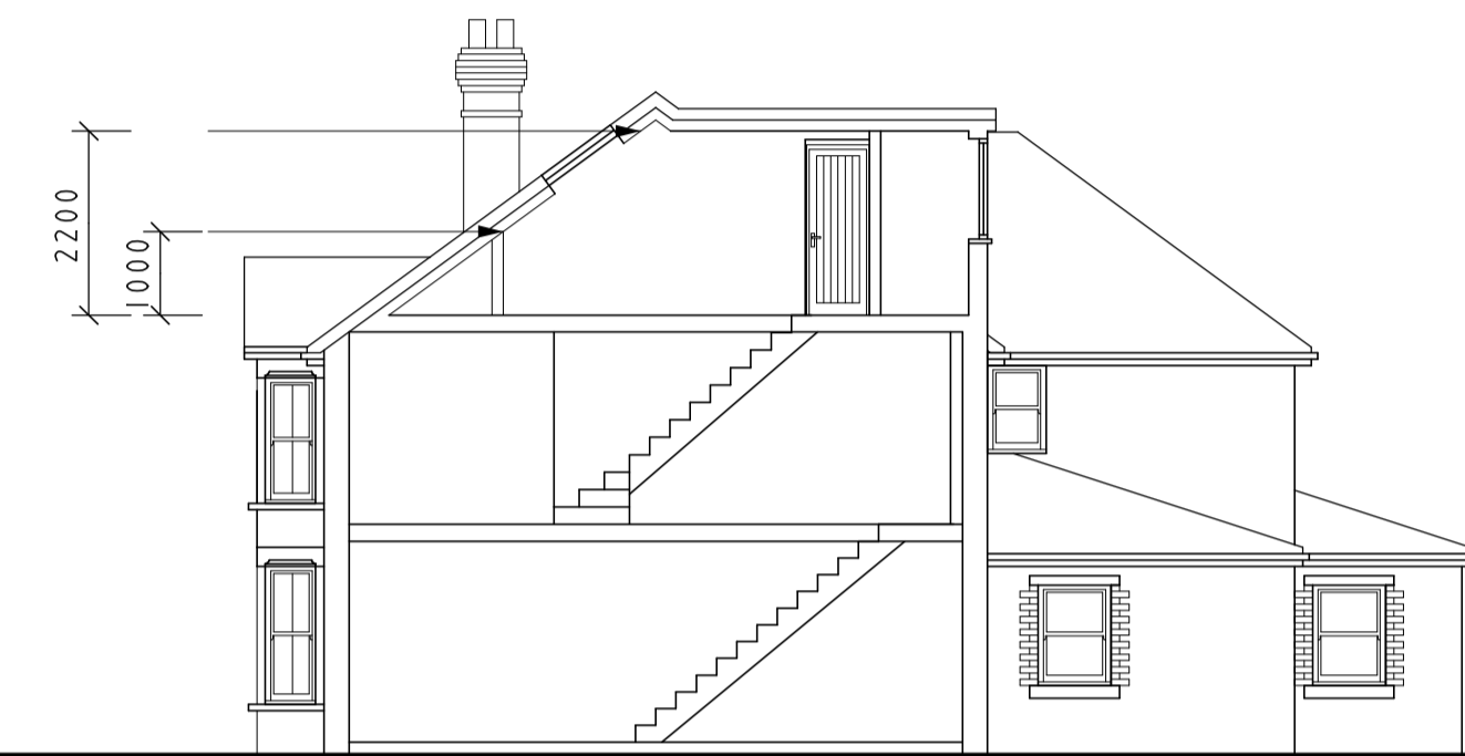
Proposed Side Section
