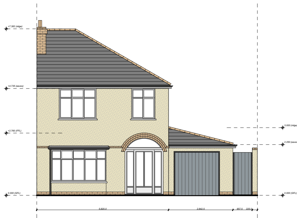
FRONT ELEVATION (NORTH)
