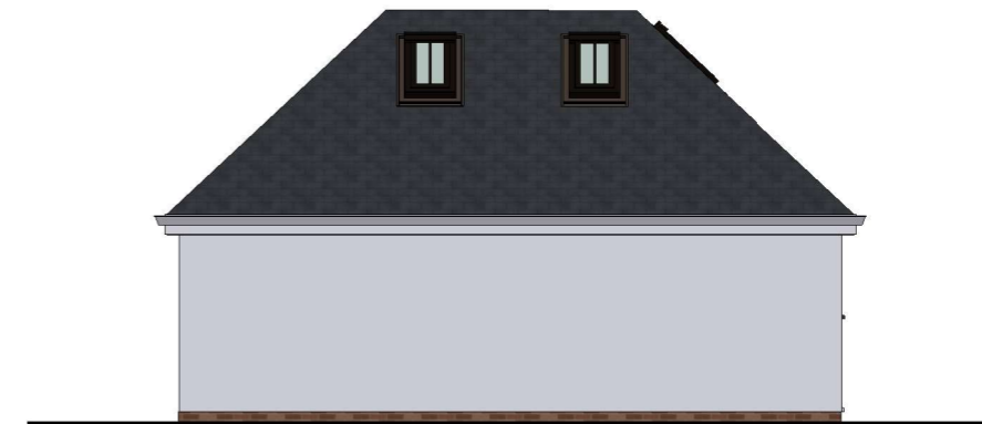
4 West Elevation 1 : 100
