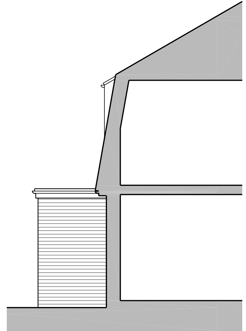
EAST ELEVATION
