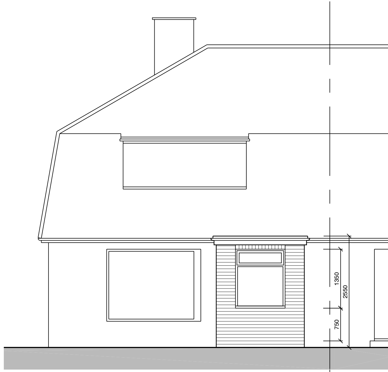
SOUTH ELEVATION
