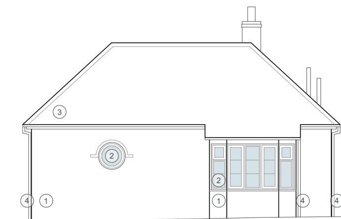
39.0m DATUM EAST ELEVATION
