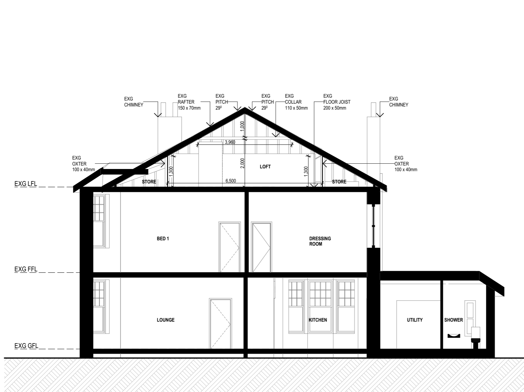
EXISTING SECTION 01
