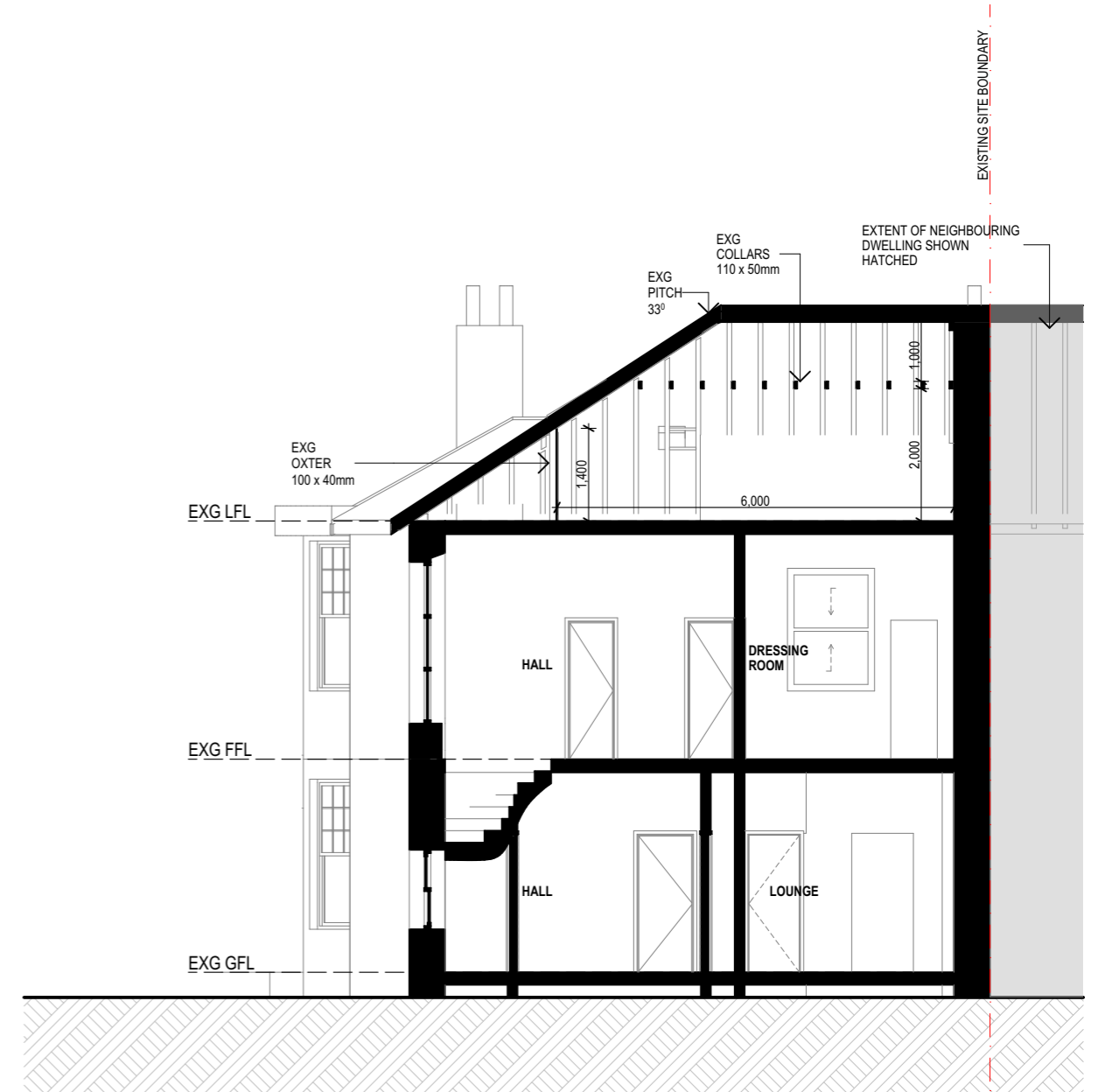
EXISTING SECTION 02
