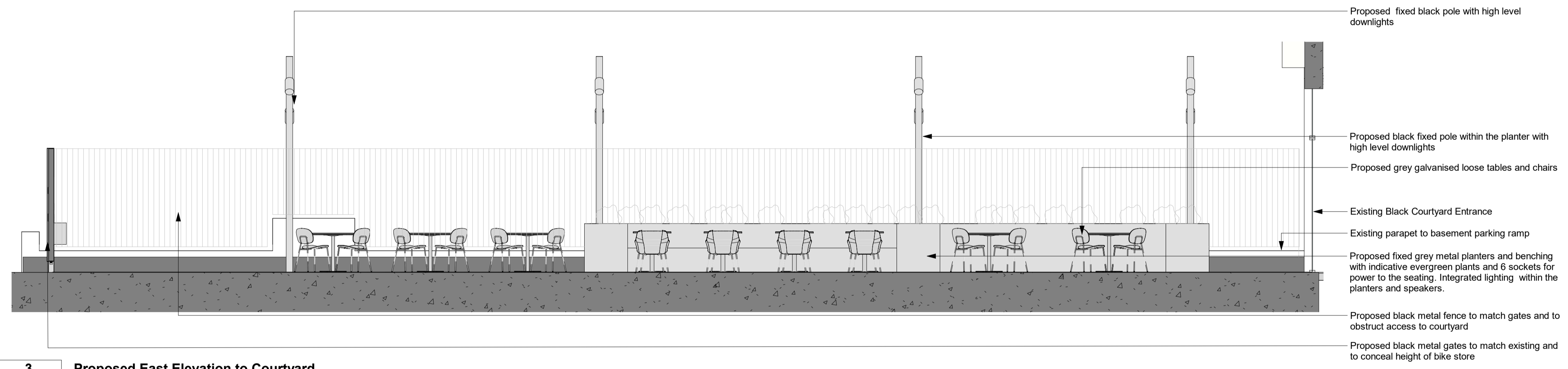
3 Proposed East Elevation to Courtyard 366 1 : 50
