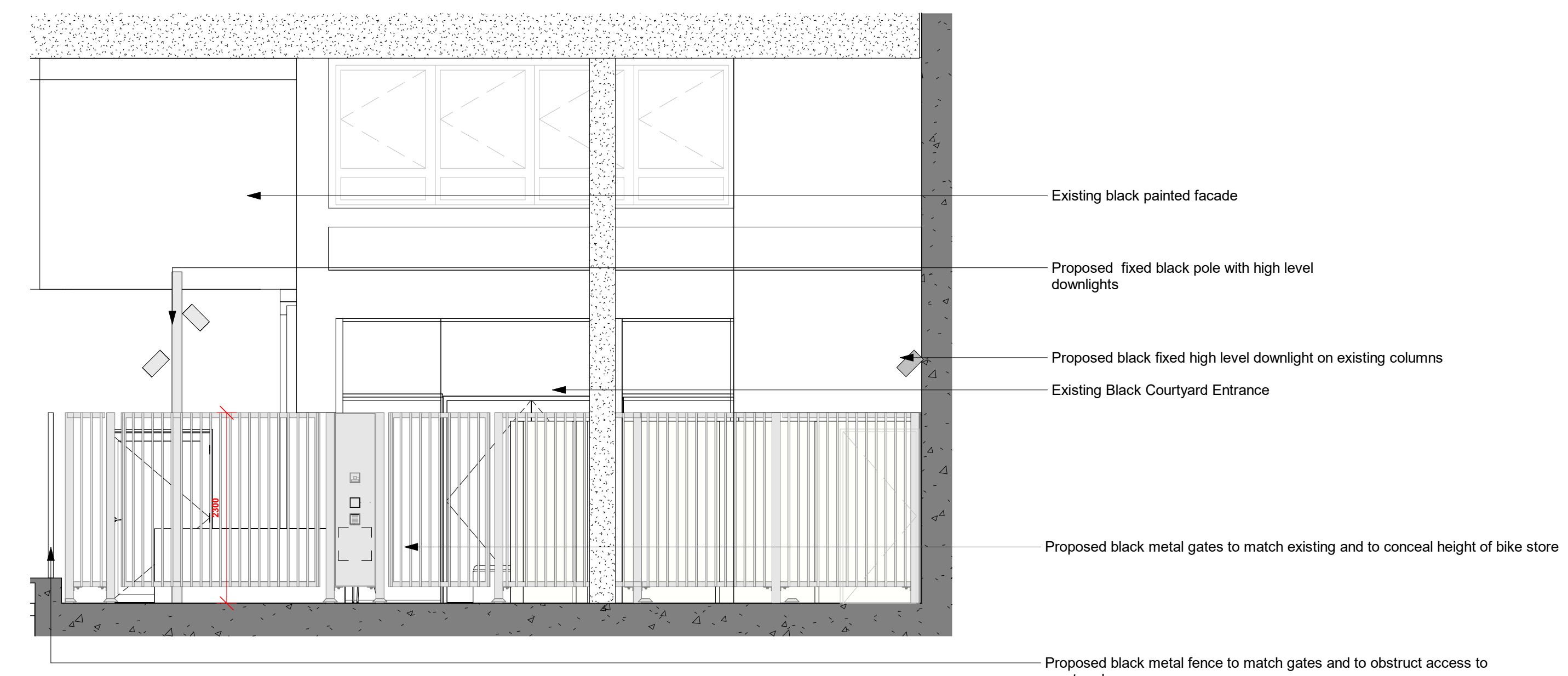
1 Proposed Gate Elevation 363 1 : 50
