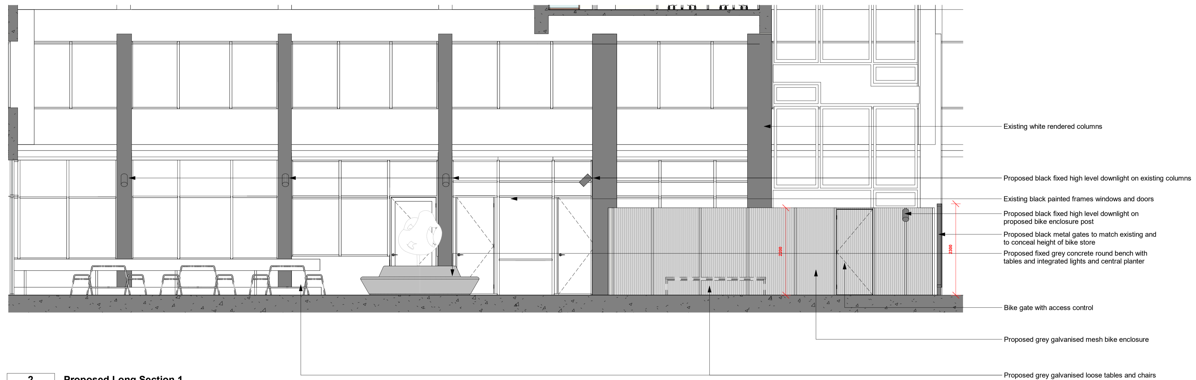
2 Proposed Long Section 1 365 1 : 50
