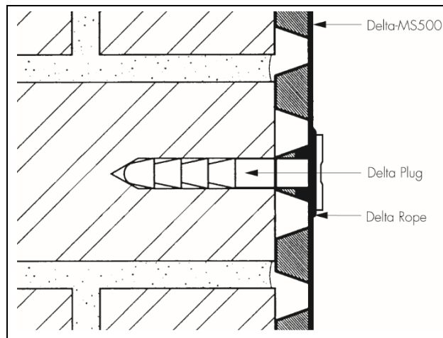
Figure 2 Delta Plug fixing detail
