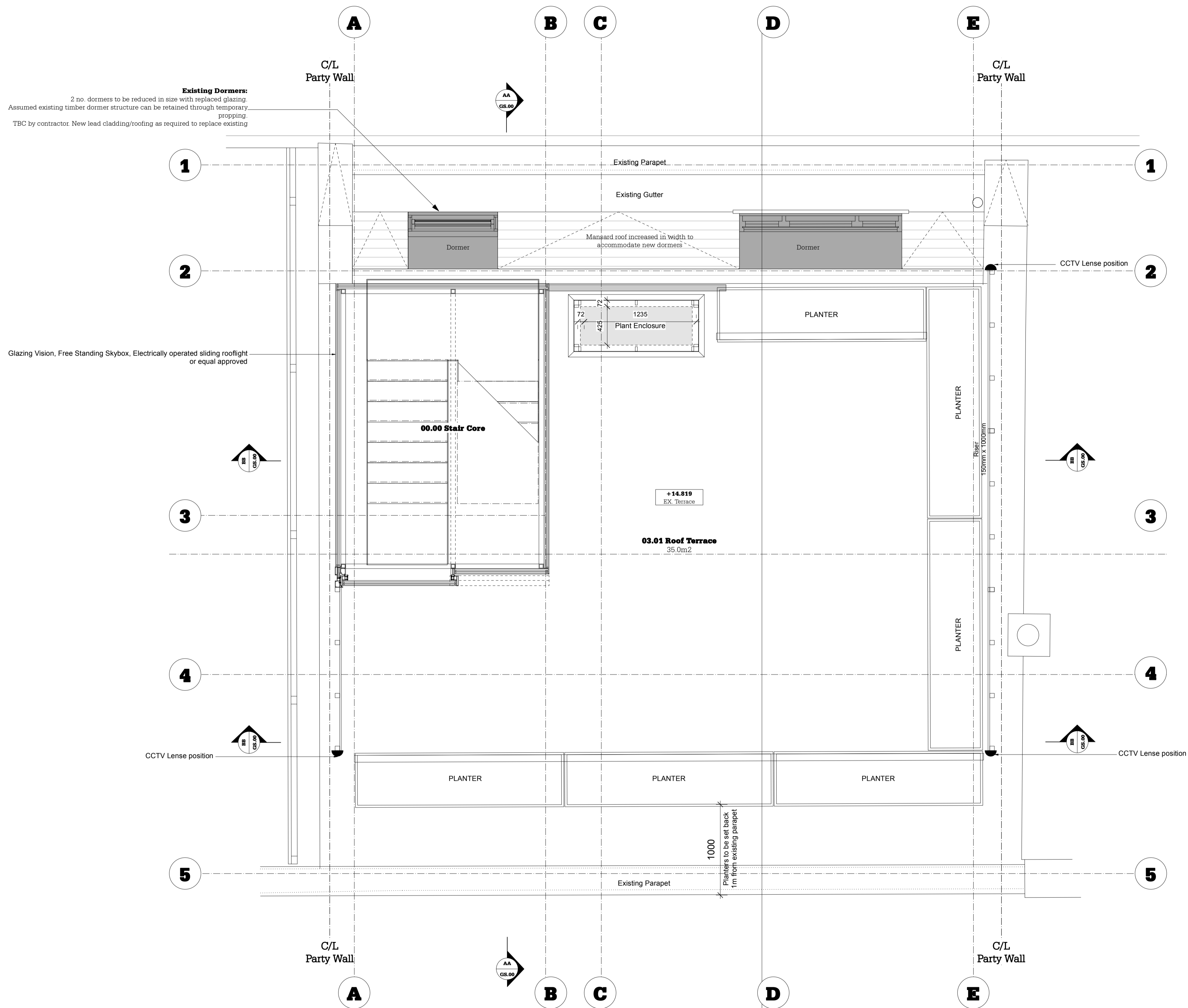
1 Roof Terrace Proposed GA.05 1:25 @ A1
