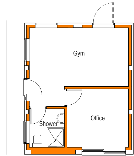
Proposed Garage Floor Plan
