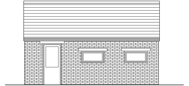
Existing Side Garage Elevation
