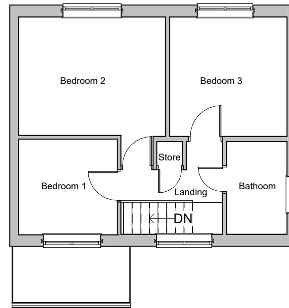
05. FF - FFL Proposed 1 : 100
