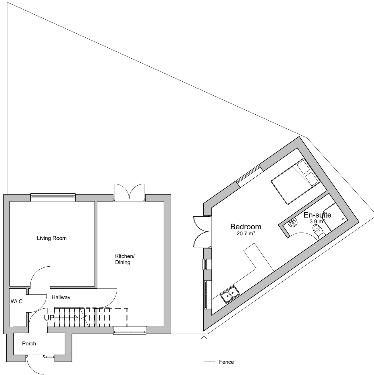
01. GF - FFL Proposed 1 : 100
