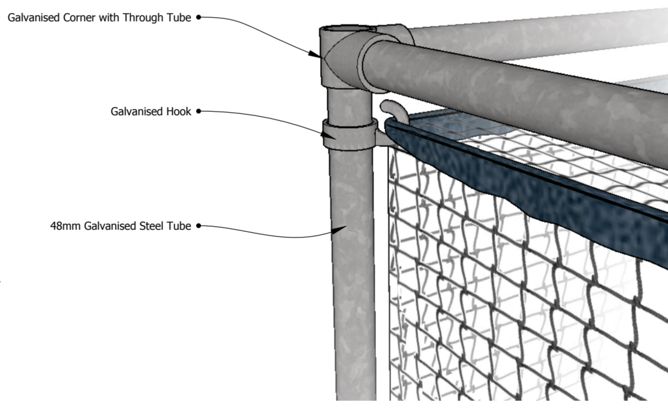
TOP CORNER DETAIL scale: NTS EN08 04
