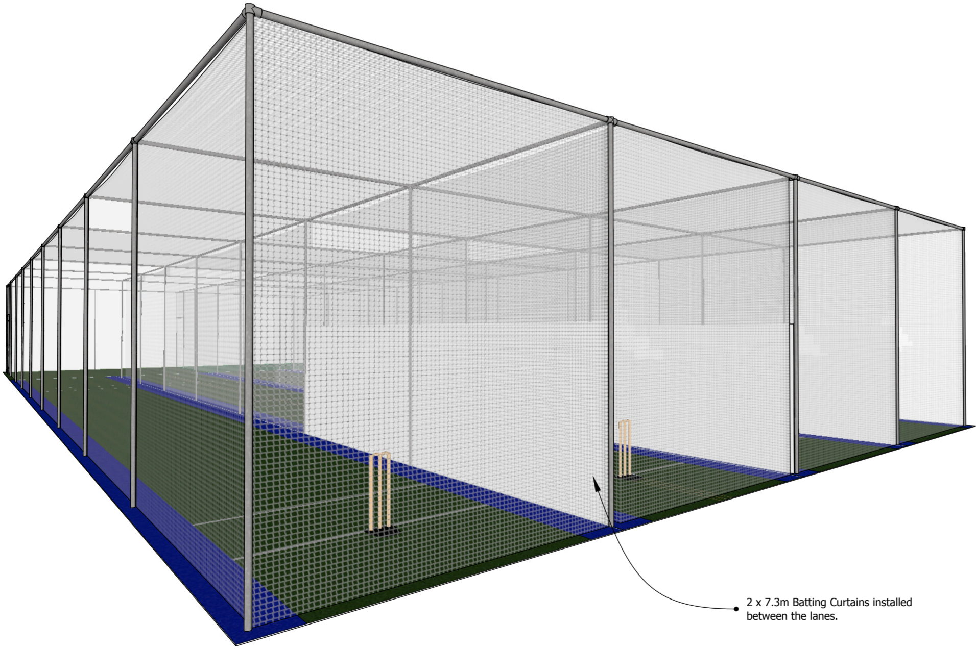
FRONT PERSPECTIVE 2 scale: NTS EN08 02
