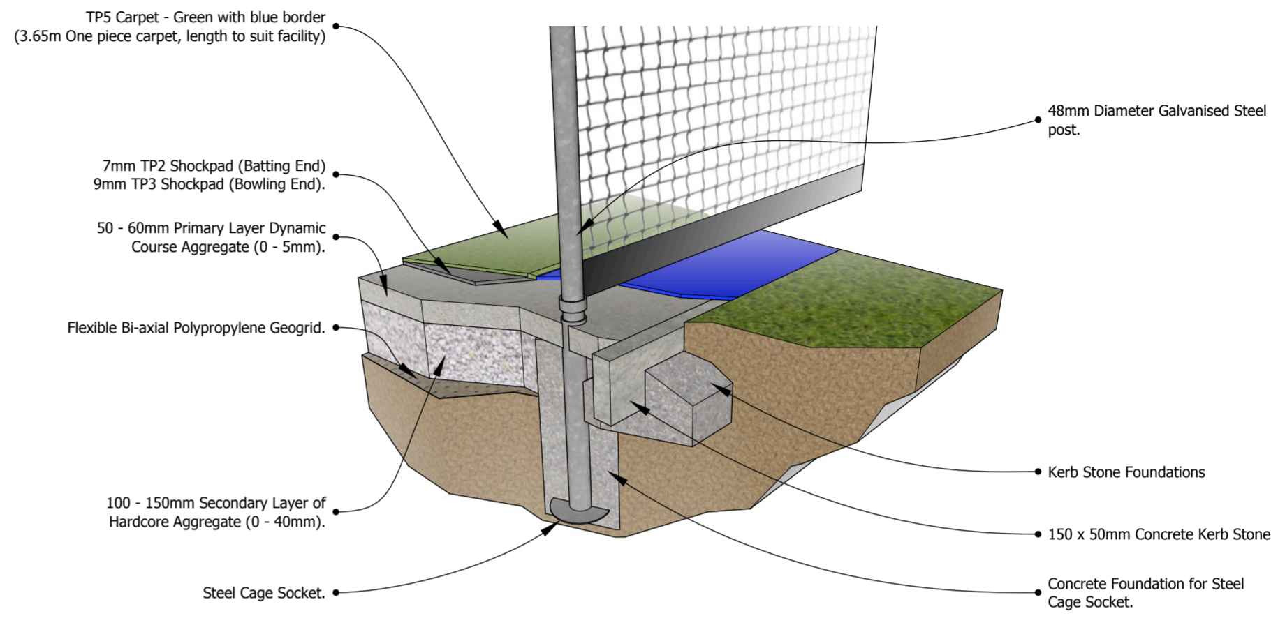
CAGE POST INSTALLATION scale: NTS EN08 03
