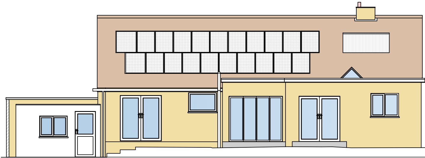
REAR (SOUTH)
