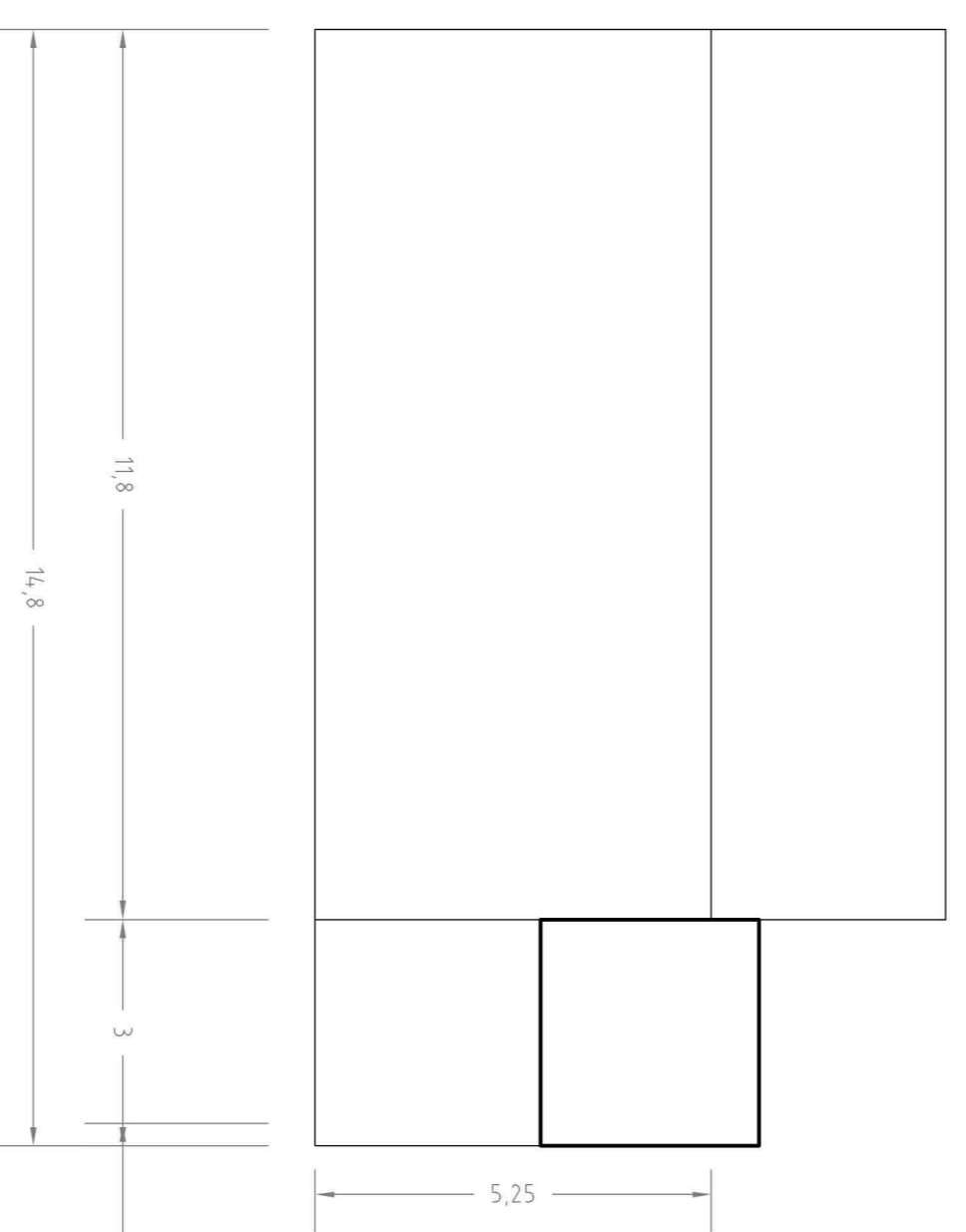
East Elevation
