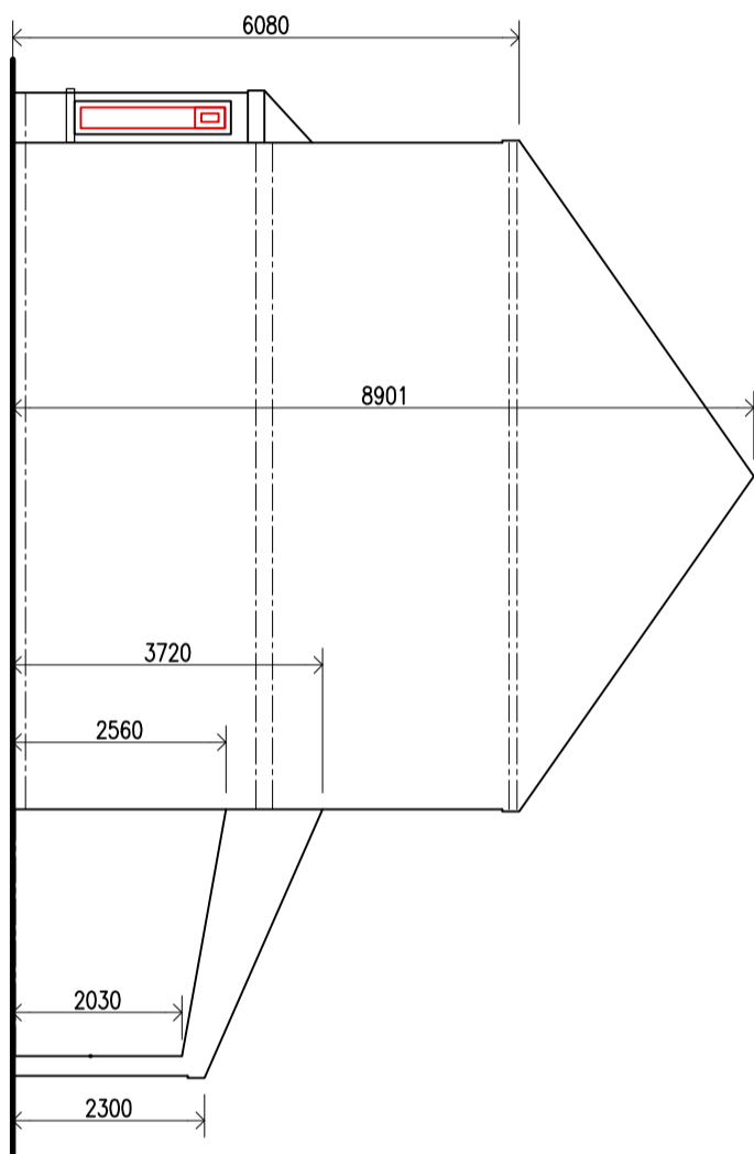
EXISTING SIDE SECTIONAL ELEVATION. (1:100)
